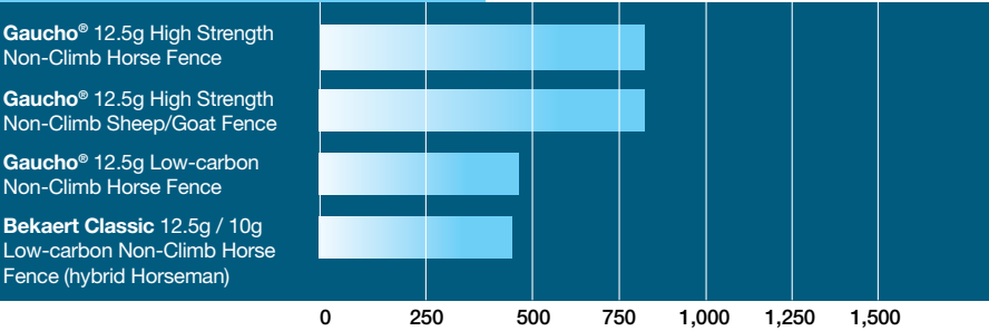
Woven Wire Breaking Strength (in pounds)
