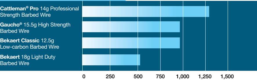
Barbed Wire Breaking Strength (in pounds)
