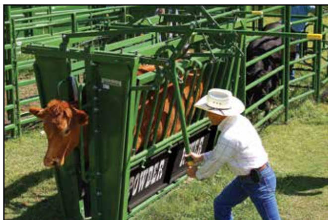
M2000 Manual Chute With Stabilizer Order No. 002-51500
