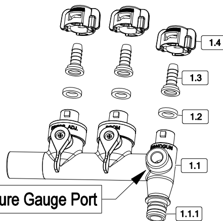
Manifold Detail #5281538
