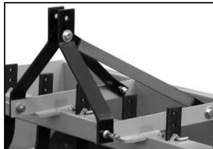
A-Frame correctly assembled with lift pins and front lift arms on the outside of horizontal angles
