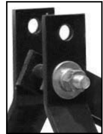
A-Frame correctly assembled with lift pins and front lift arms on the outside of horizontal angles
